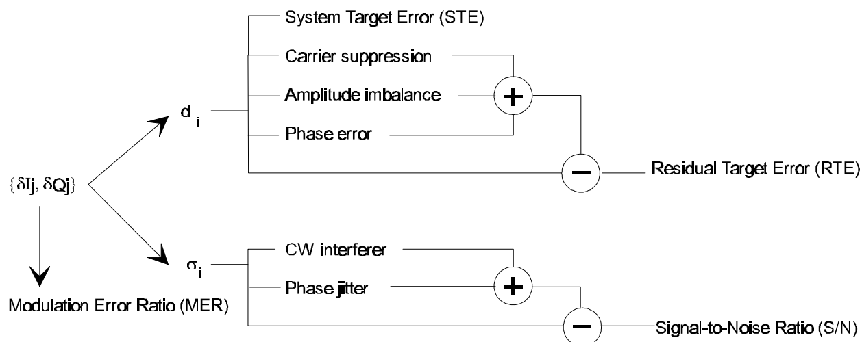
Figure 5: Relationship between the parameters describing different IQ distortions
