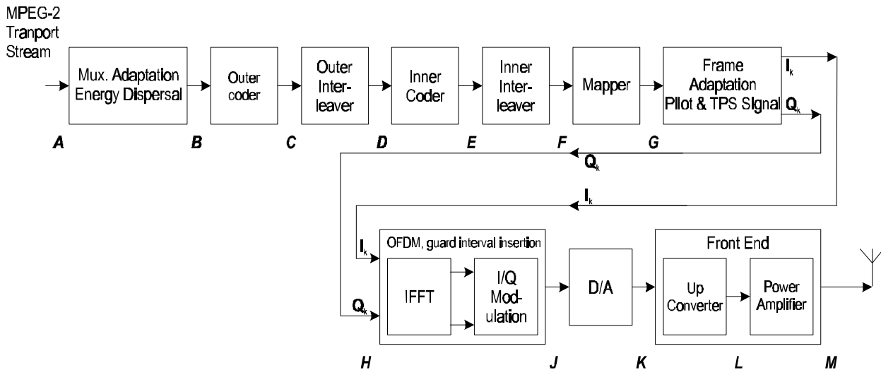
Figure 12: Block diagram of a DVB-T transmitter
