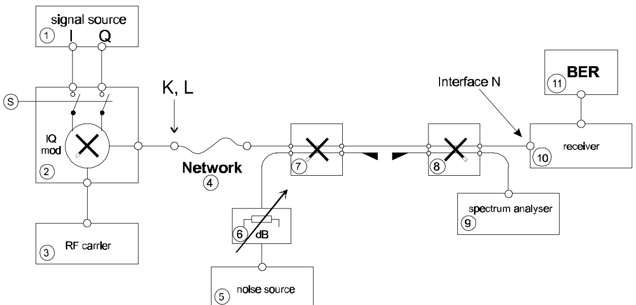
Figure E.12: BER vs. C/N by variation of Gaussian noise power
