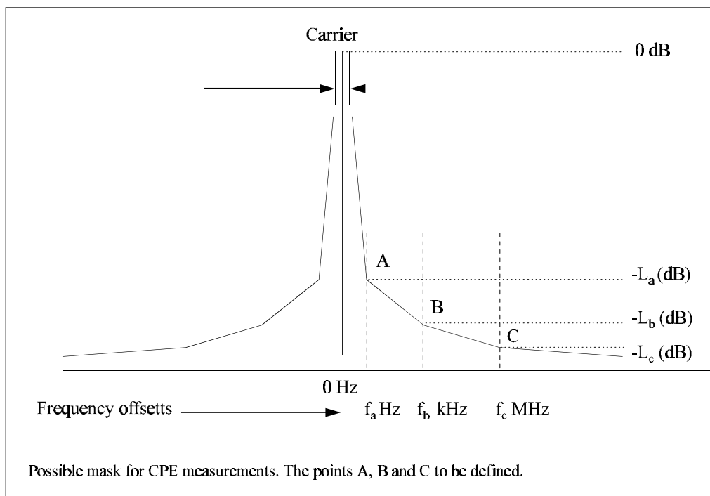
Figure 14: Possible mask for CPE measurements
