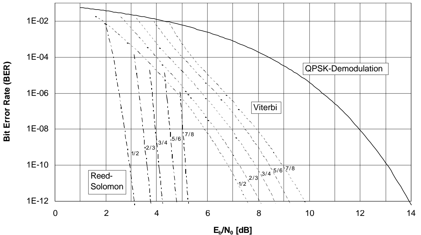
Figure G.2: BER for DVB satellite transmission
