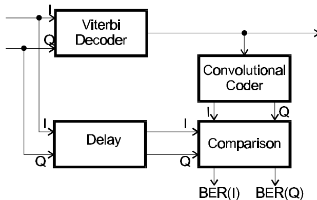
Figure 11: BER measurement before Viterbi decoding
