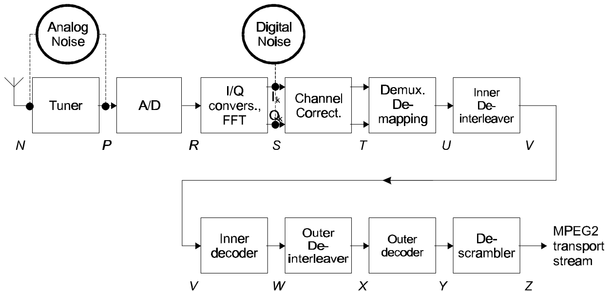
Figure 13: Block diagram of a DVB-T receiver
