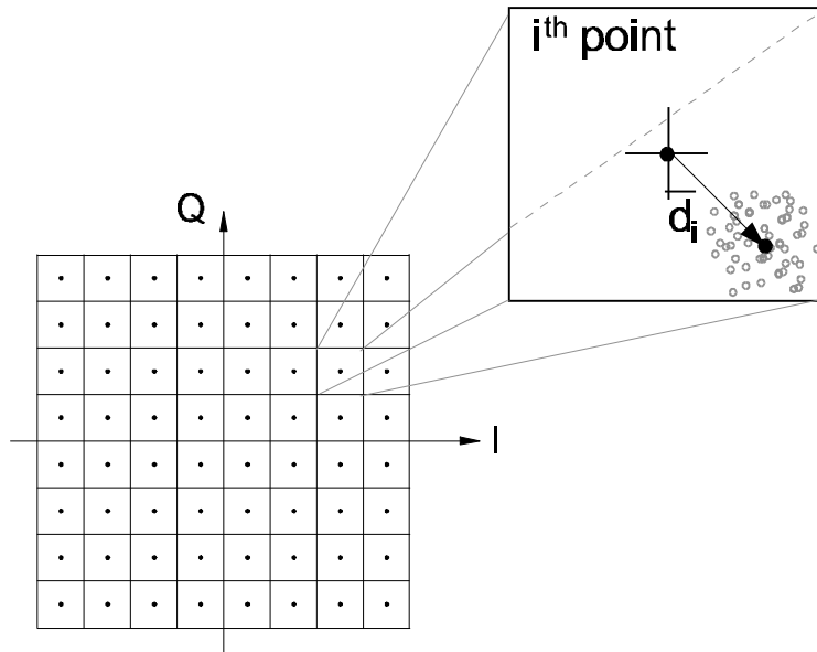
Figure 6: Definition of Target Error Vector (TEV)
