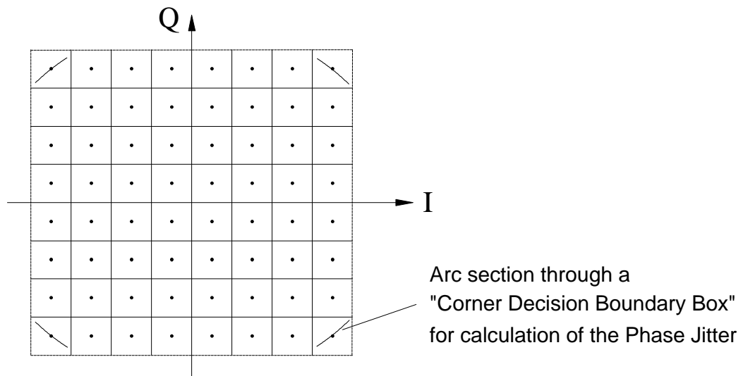
Figure 18: Position of "Arc section" in the constellation diagram to define PJ (example: 64-QAM)
