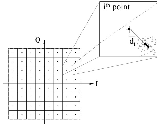
Figure 16: Definition of Target Error Vector (TEV)
