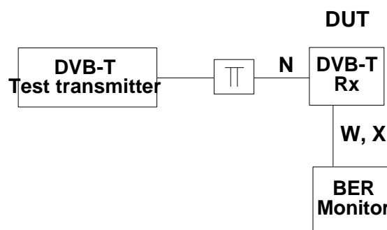
Figure E.6: Receiver sensitivity/dynamic range for a Gaussian channel
